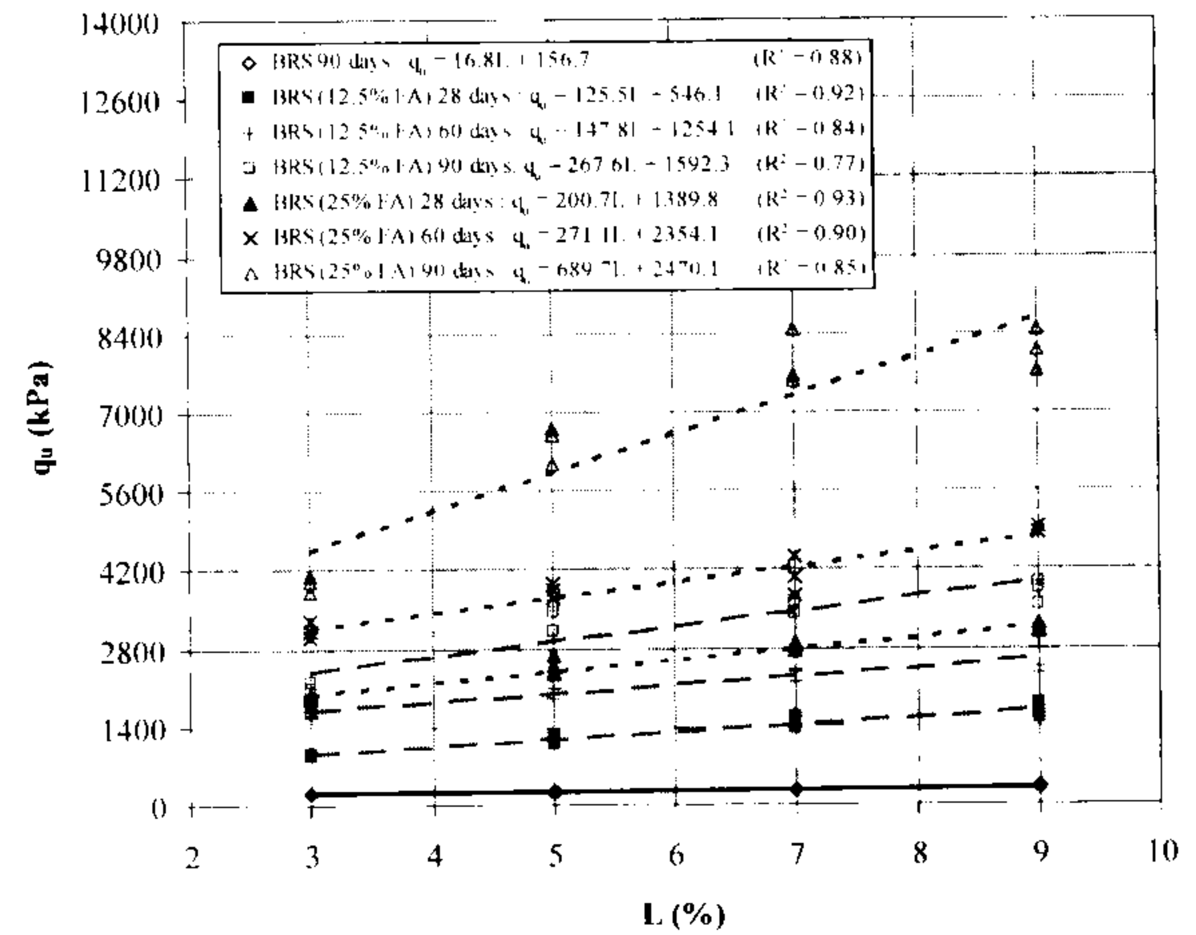
Fig. 4. Variation of unconfined compressive strength of BRS, BRS (12.5% FA) and BRS (25% FA) with lime content considering \gamma_d = 17 \text{ kN/m}^3 and 28, 60 and 90 days curing specimens
