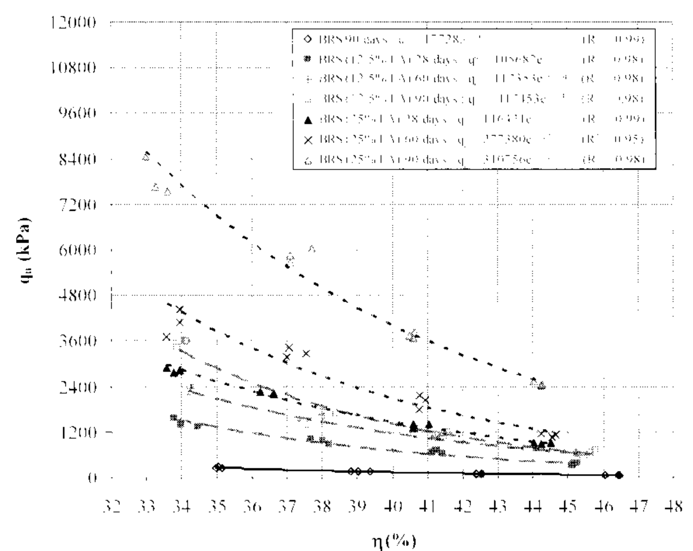
Fig. 6. Variation of unconfined compressive strength of BRS-lime, BRS (12.5% FA)-lime and BRS (25% FA)-lime with porosity considering L = 7\% and 28, 60 and 90 days curing specimens
