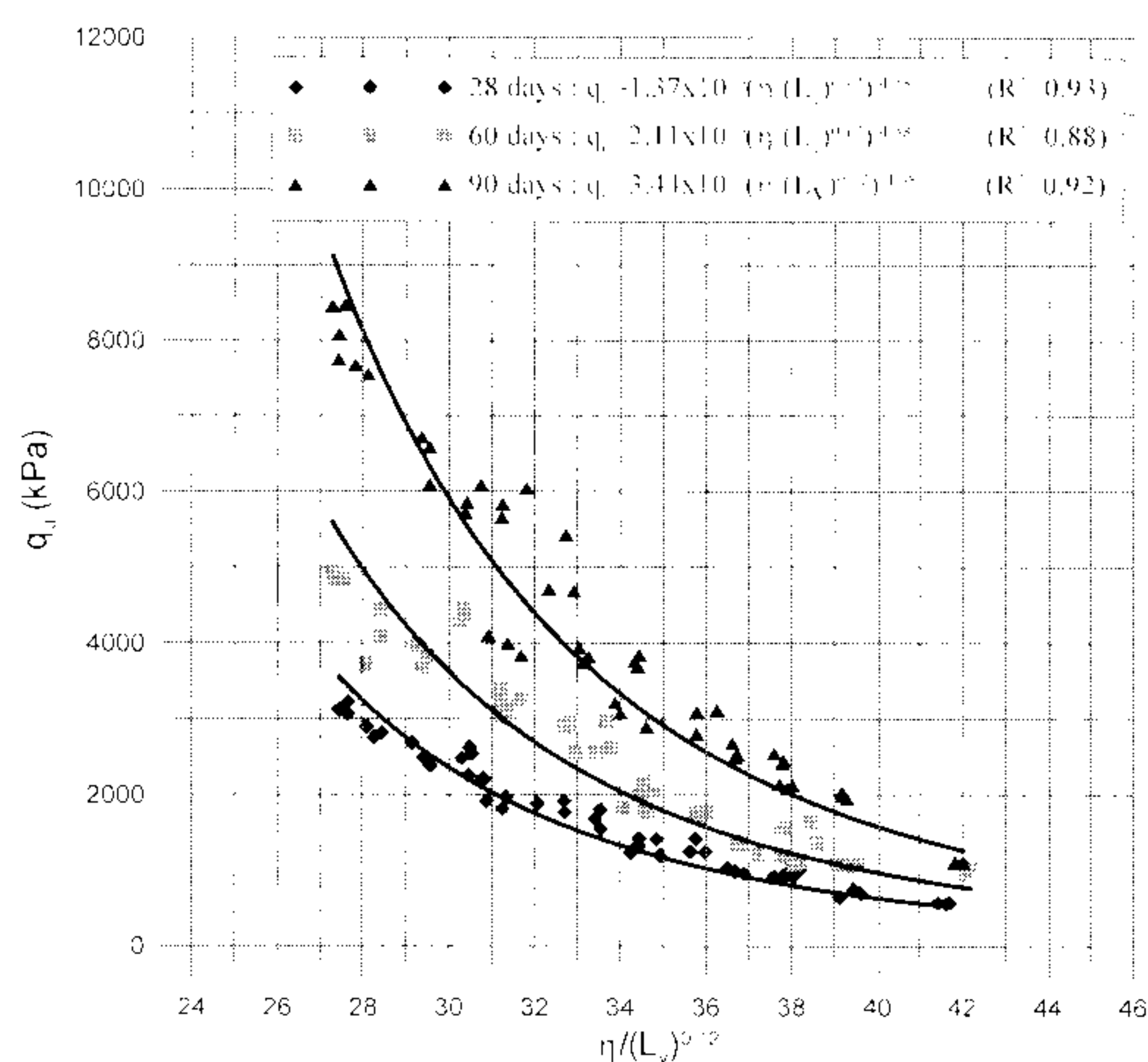
Fig. 10. Variation of unconfined compressive strength of BRS (25% FA)-lime specimens with adjusted porosity/volumetric content of lime at 28 days, 60 days and 90 days curing periods
