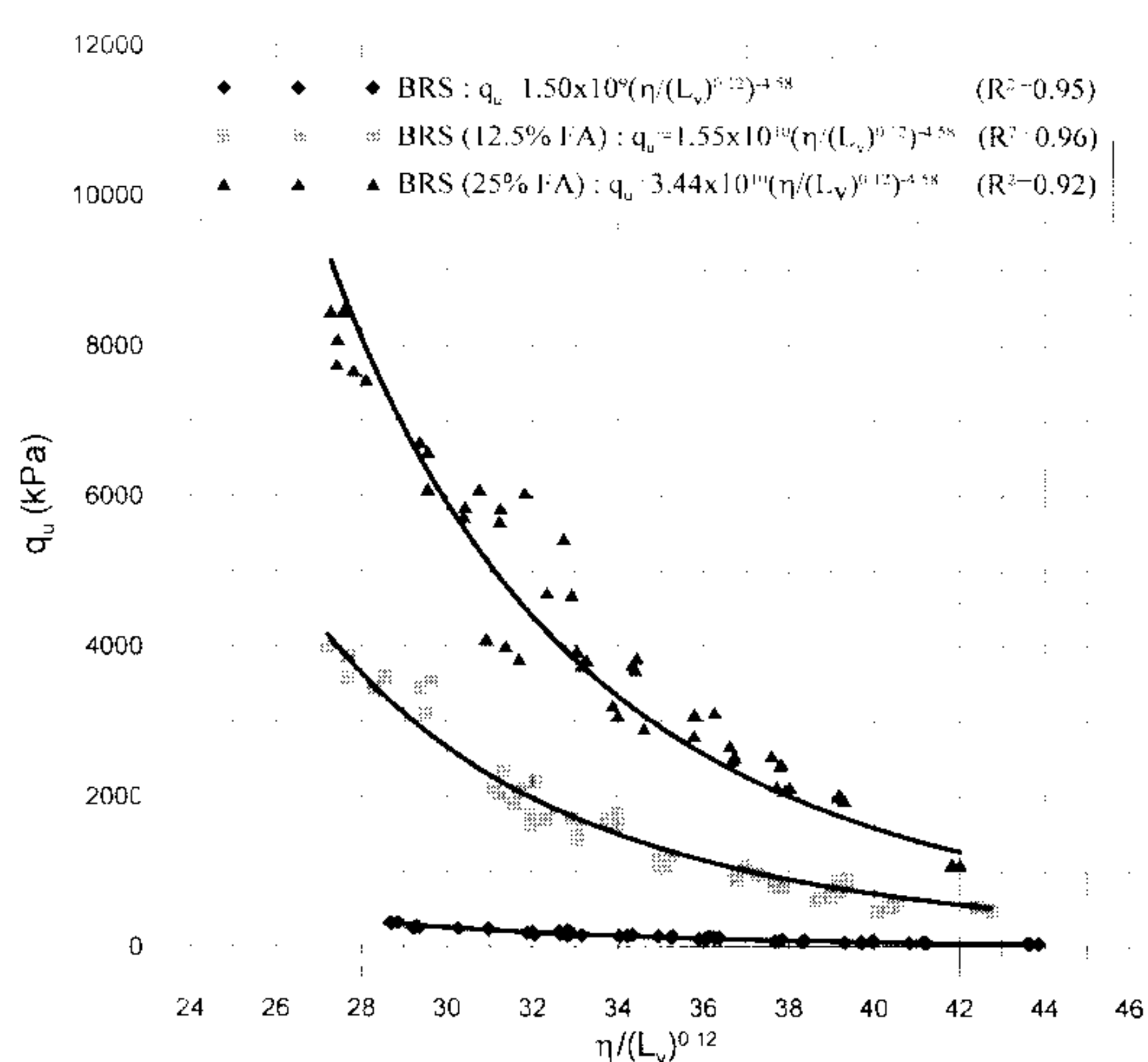
Fig. 11. Variation of unconfined compressive strength with adjusted porosity/volumetric content of lime—(curves adjusted for each one of the three FA content studied)
